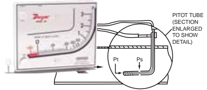
PITOT TUBE SENSES TOTAL AND STATIC PRESSURES. MANOMETER MEASURES VELOCITY PRESSURE-(DIFFERENCE BETWEEN TOTAL AND STATIC PRESSURES).
