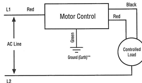
Connection Diagram for Model 105FR Control
