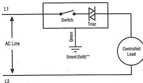
Connection Diagram for 2-Wire* Controls (Switch Models)
