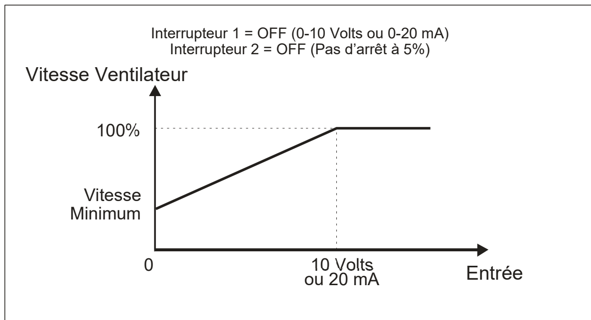
Figure 3: Diagrammes logiques (Mode Auto)
