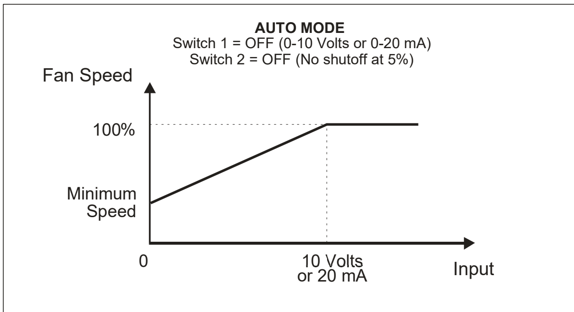
Figure 4: Logic Diagrams (Auto Mode)
