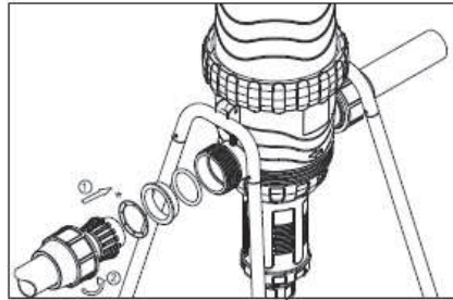
* Optional Special grip ring for P.V.C pipes
